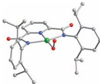
Figure 2. Calculated structure of end-on triplet Cu(II)-superoxo complex 3 . Carbon (gray), nitrogen (blue), oxygen (red), and copper (green) are shown. Hydrogens omitted for clarity.
