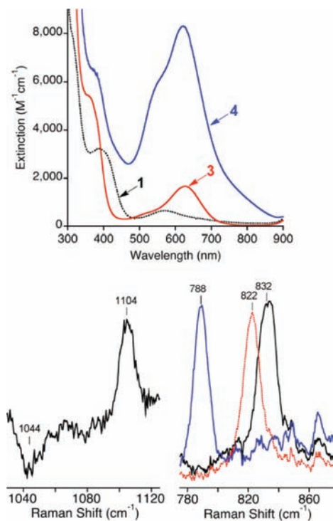
Figure 1. (Top) UV-vis spectra of compounds 1 , 3 , and 4 ( -80\text{ }^{\circ}\text{C} , DMF/THF). (Bottom Left) Resonance Raman difference spectrum ( ^{16}\text{O} – ^{18}\text{O} ) for compound 3 prepared from \text{K}^{16}\text{O}_2 or \text{K}^{18}\text{O}_2 ( -196\text{ }^{\circ}\text{C} , \lambda_{\text{ex}} = 647\text{ nm} ). (Bottom Right) Resonance Raman spectra for compound 4 prepared from 3 ( ^{16}\text{O} ) (black line) or 3 ( ^{18}\text{O} ) (blue line), overlaid with spectrum of [(tmpa) 2 Cu 2 ( ^{16}\text{O}_2 )](OTf) 2 (red dotted line) ( -196\text{ }^{\circ}\text{C} , \lambda_{\text{ex}} = 647.1\text{ nm} ).
